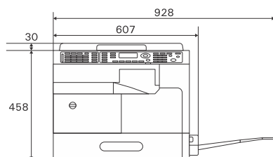
bizhub 226 (206) + OC-512
