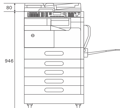
Front View bizhub 306/266 + DF-625 + PF-509 x4 + DK-708
