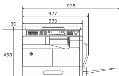
Front View bizhub 306/266 + OC-512
